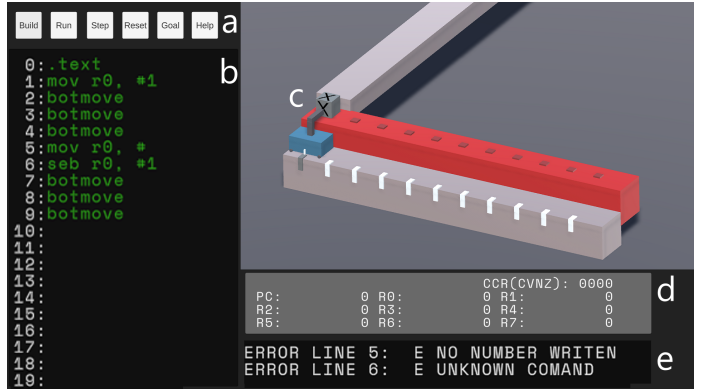
Fig. 2. Assembly Academy's user interface during one of the levels.
